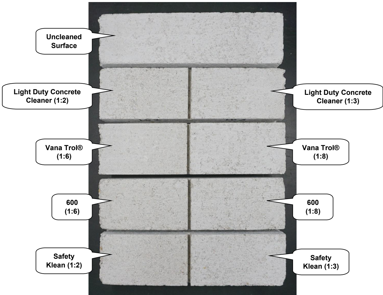
"Phoenix" Concrete Brick After Cleaning
