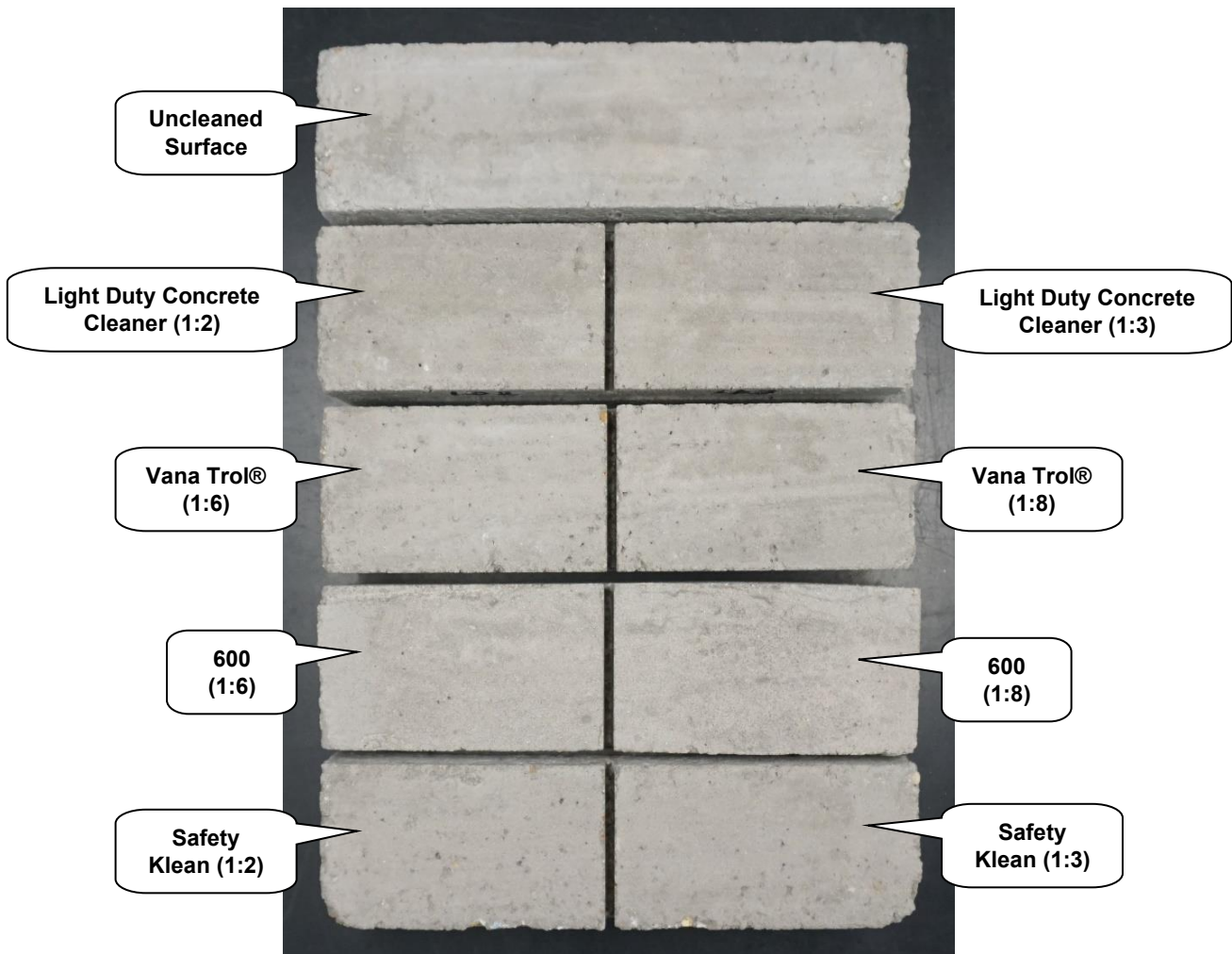
"Gray Mist" Concrete Brick After Cleaning
