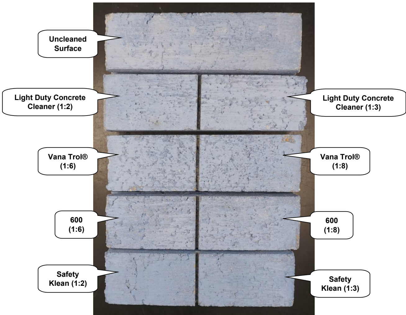
"Caribbean Blue" Concrete Brick After Cleaning
