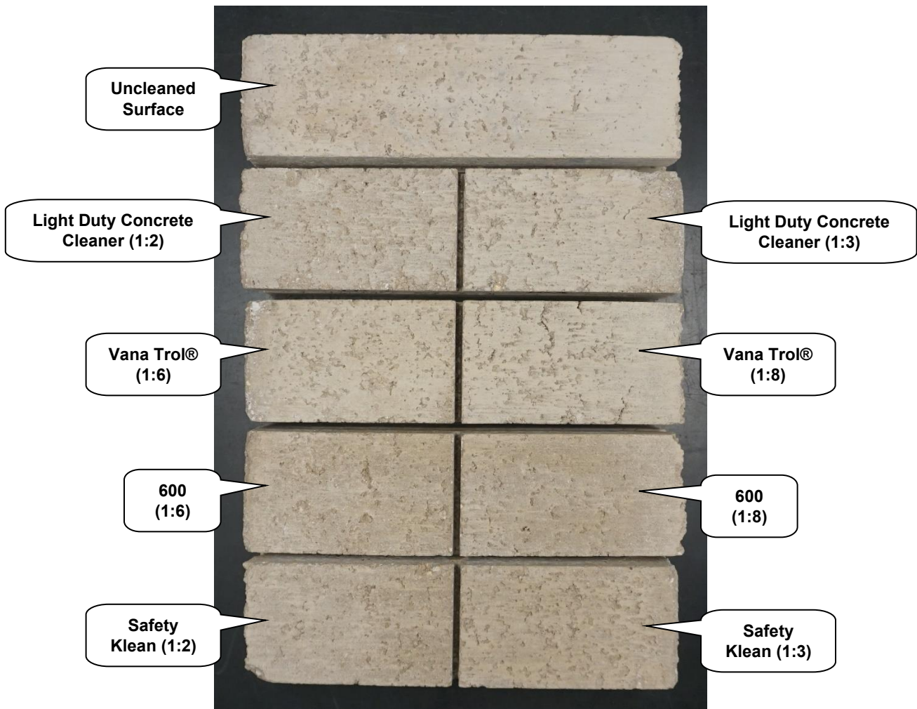
"Dune" Concrete Brick After Cleaning
