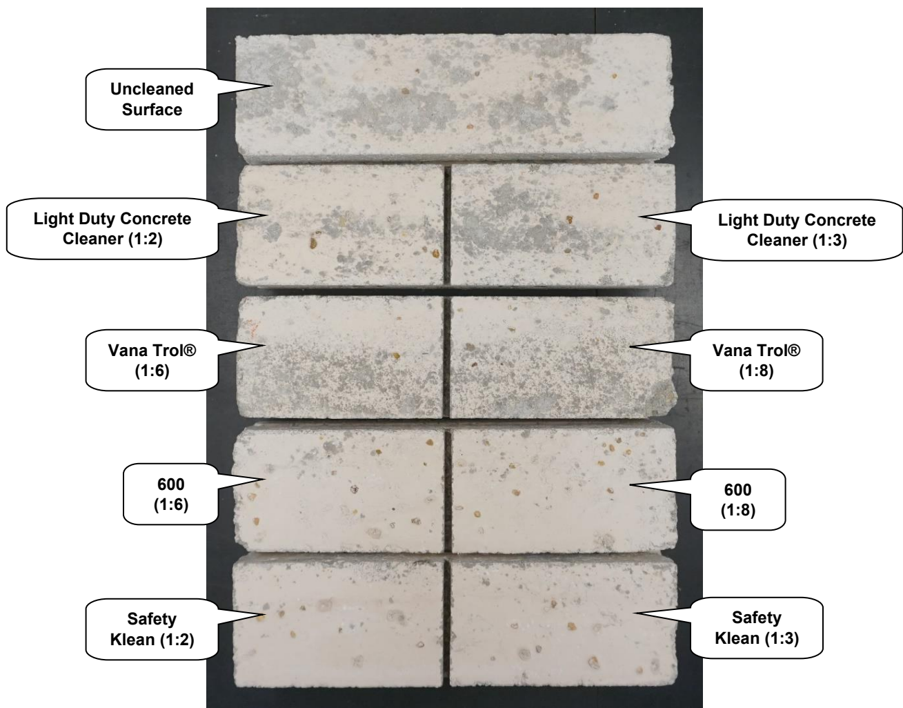
"Bristol" Concrete Brick After Cleaning
