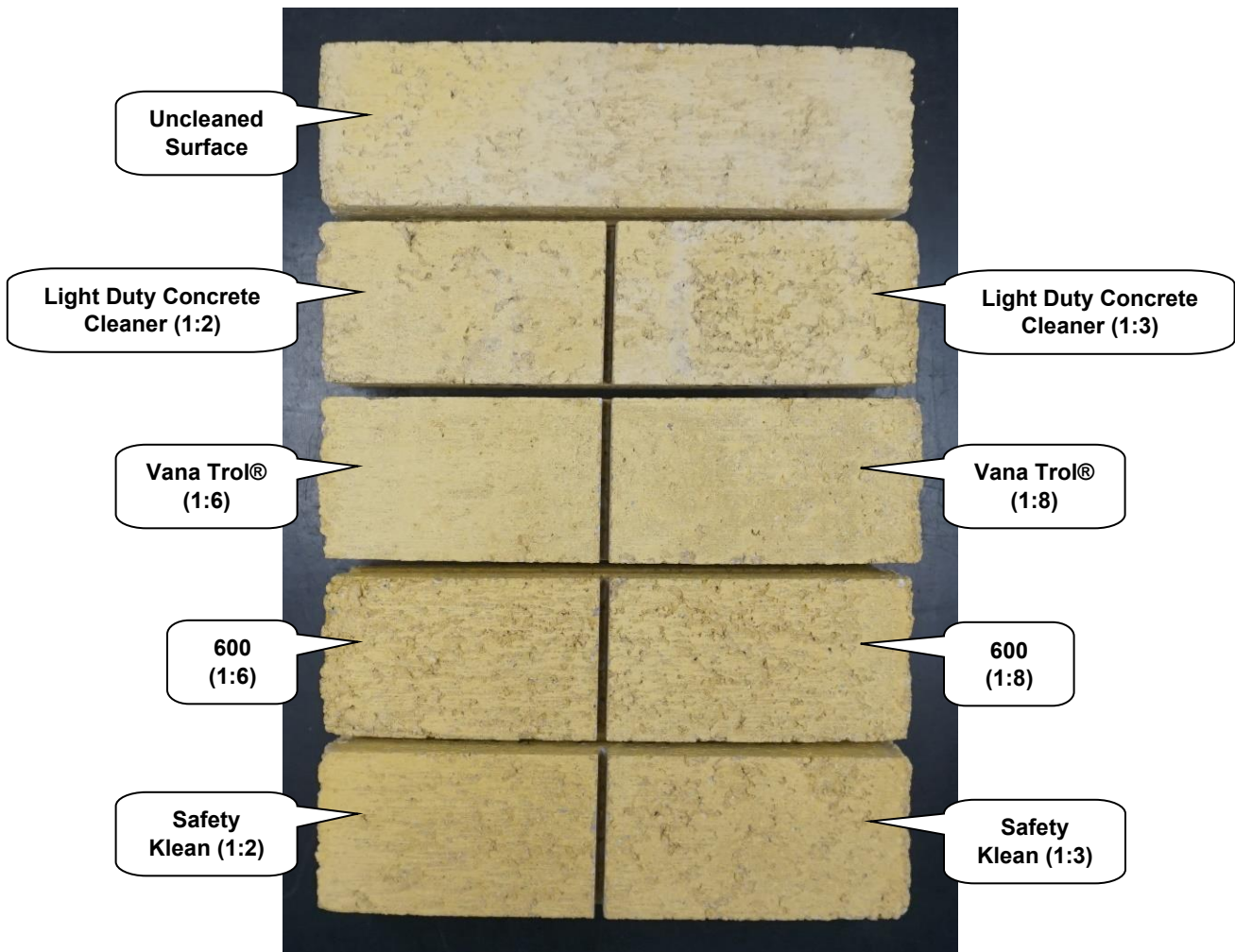
"Mustard Yellow" Concrete Brick After Cleaning
