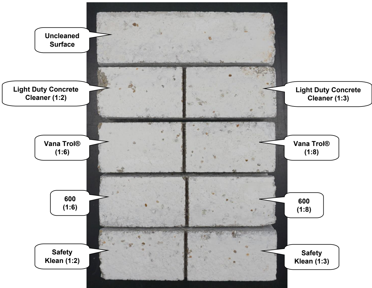
"Everest" Concrete Brick After Cleaning
