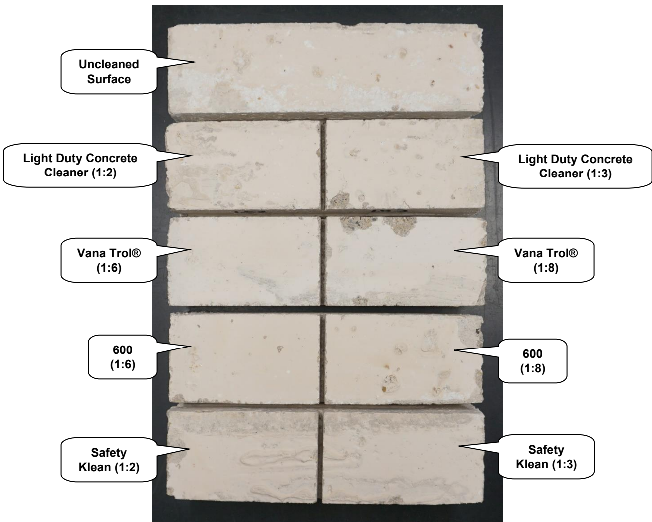
"Wheaton" Concrete Brick After Cleaning
