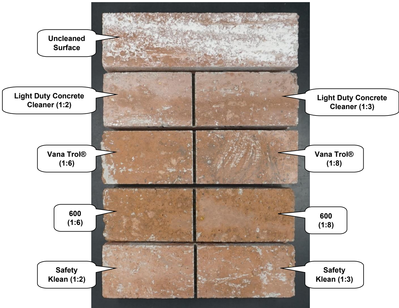
"Williamsburg" Concrete Brick After Cleaning
