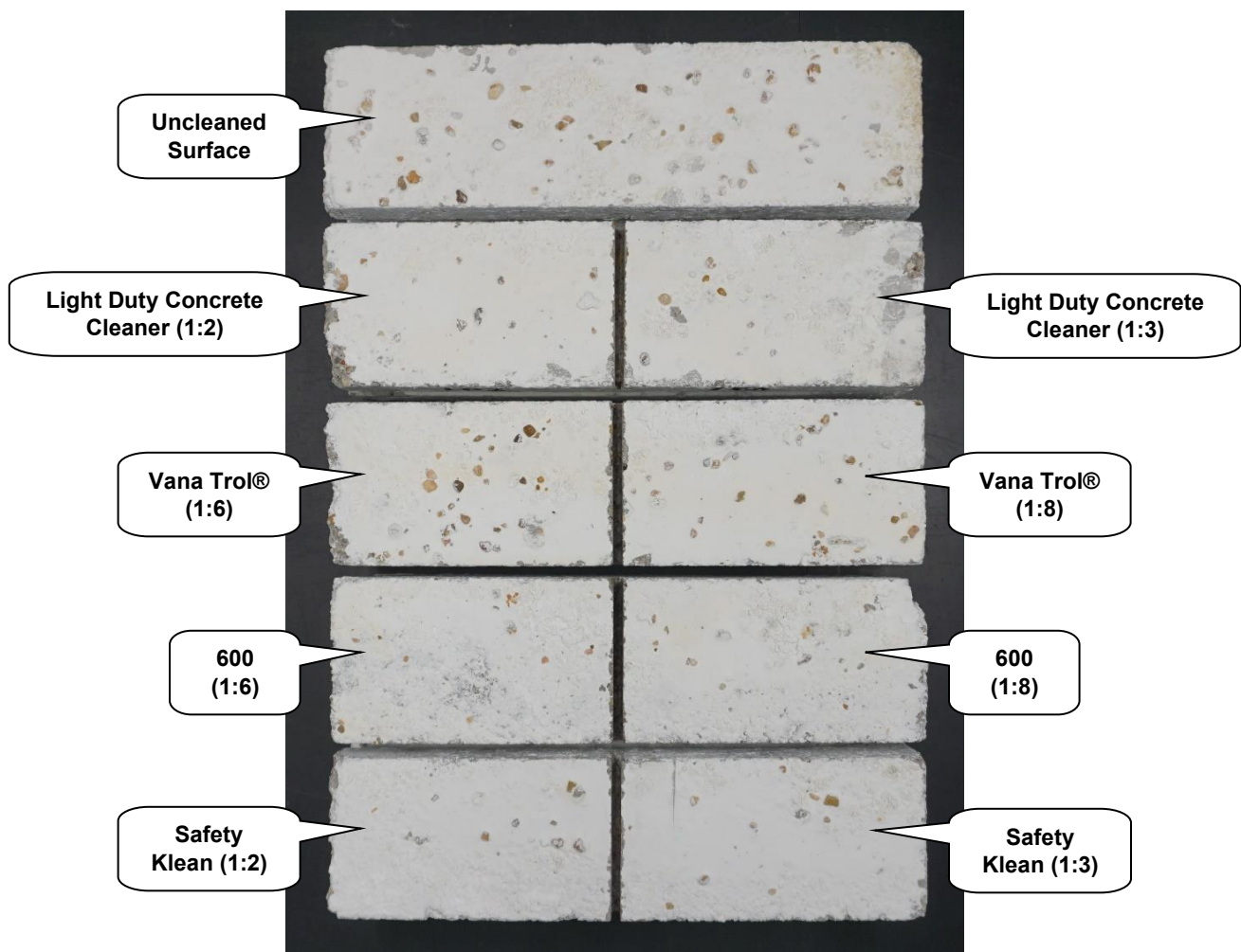
"Winter Ash" Concrete Brick After Cleaning
