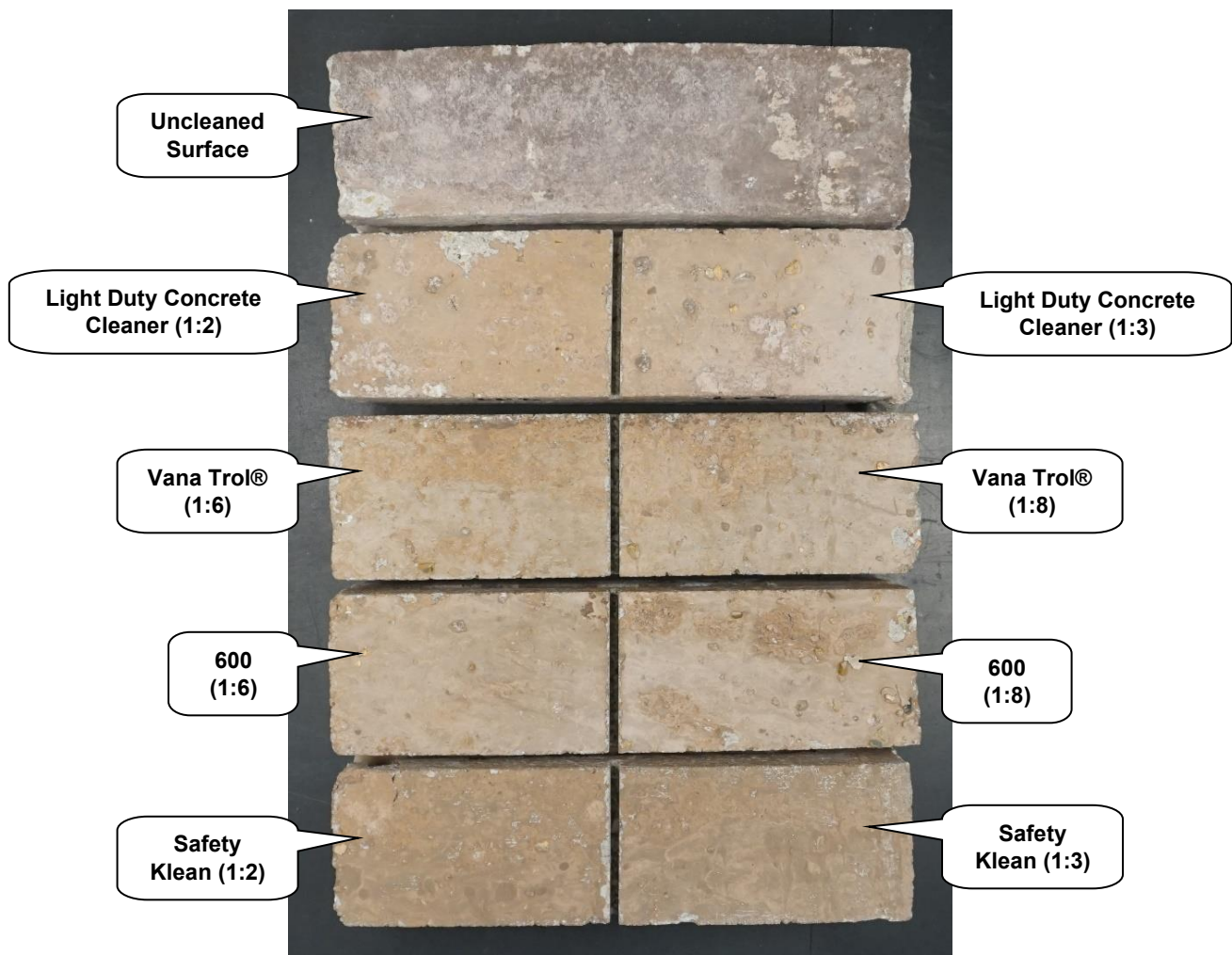
"Georgetown" Concrete Brick After Cleaning
