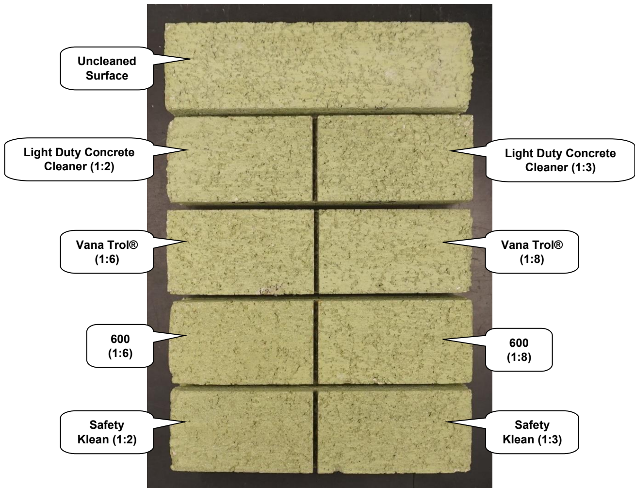
"Lime Green" Concrete Brick After Cleaning
