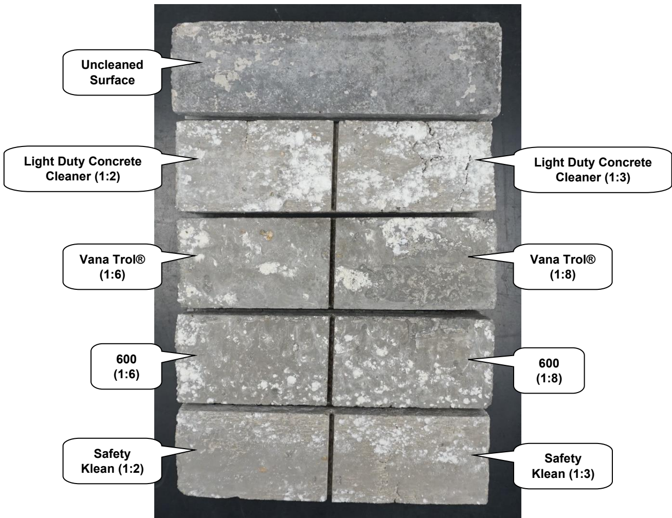
"Gettysburg" Concrete Brick After Cleaning
