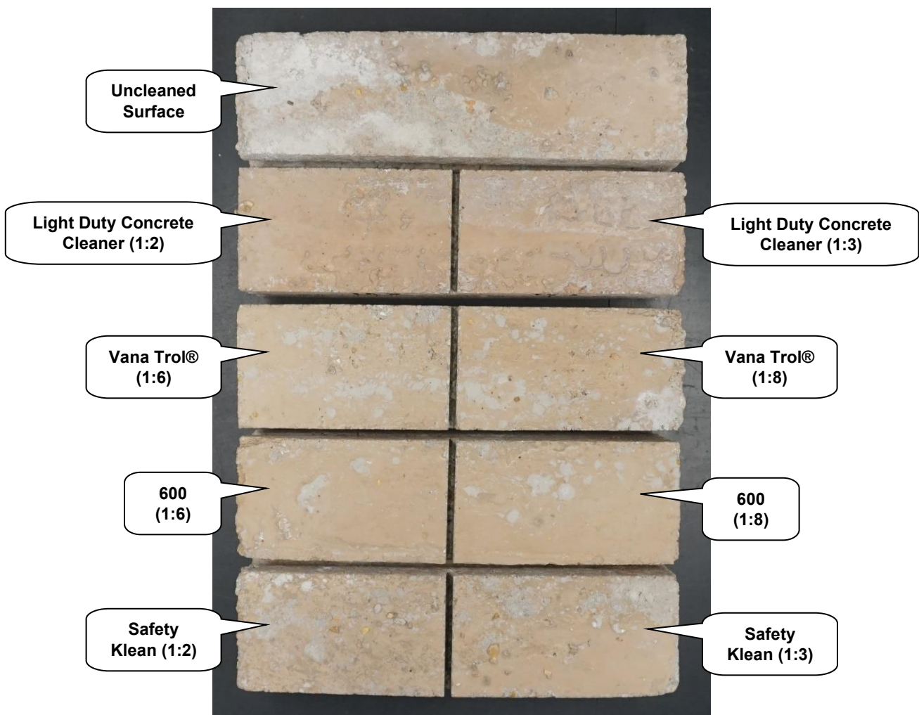
"Sahara" Concrete Brick After Cleaning
