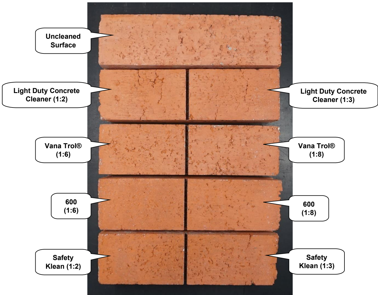
"Longhorn Orange" Concrete Brick After Cleaning
