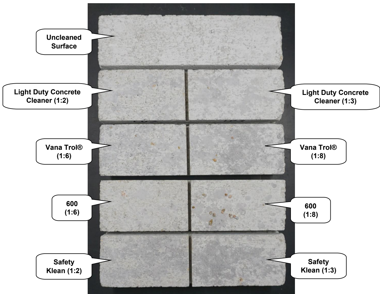
"Frost" Concrete Brick After Cleaning
