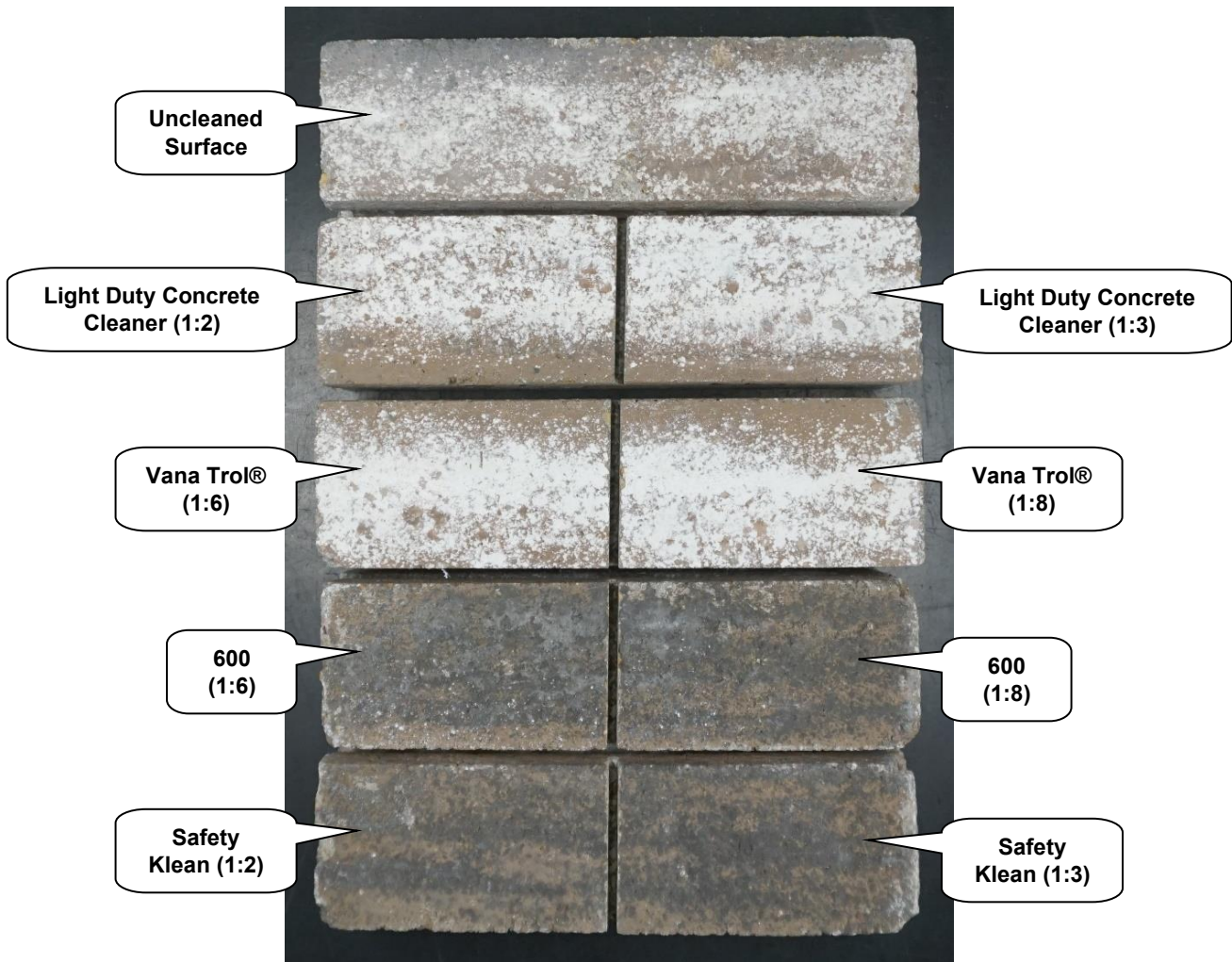
"Westfield" Concrete Brick After Cleaning
