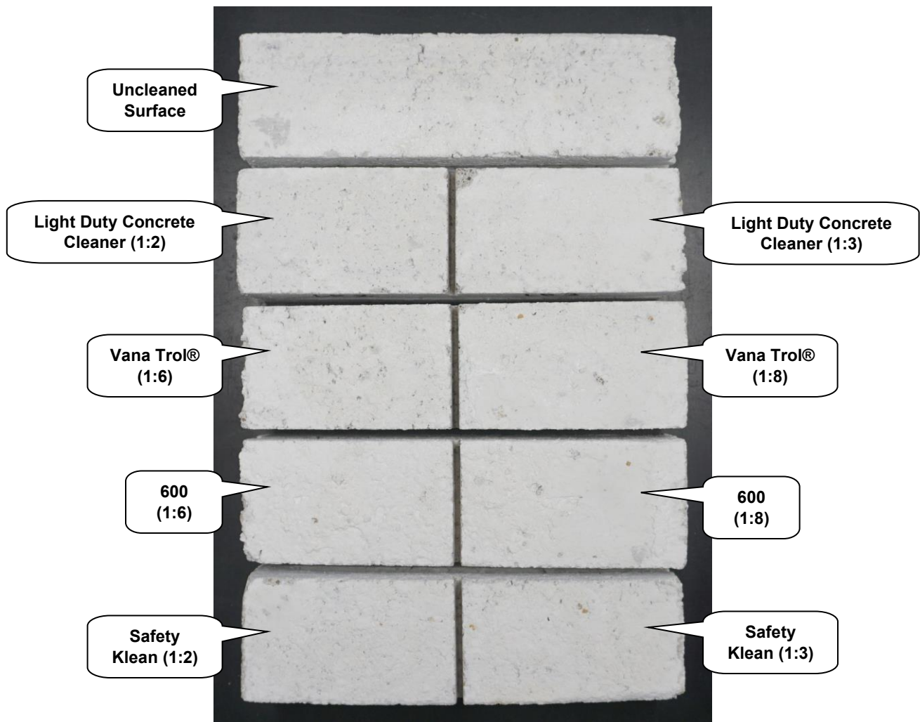
"Stardust" Concrete Brick After Cleaning
